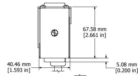
ASSEMBLY - VIEW FROM FRONT
