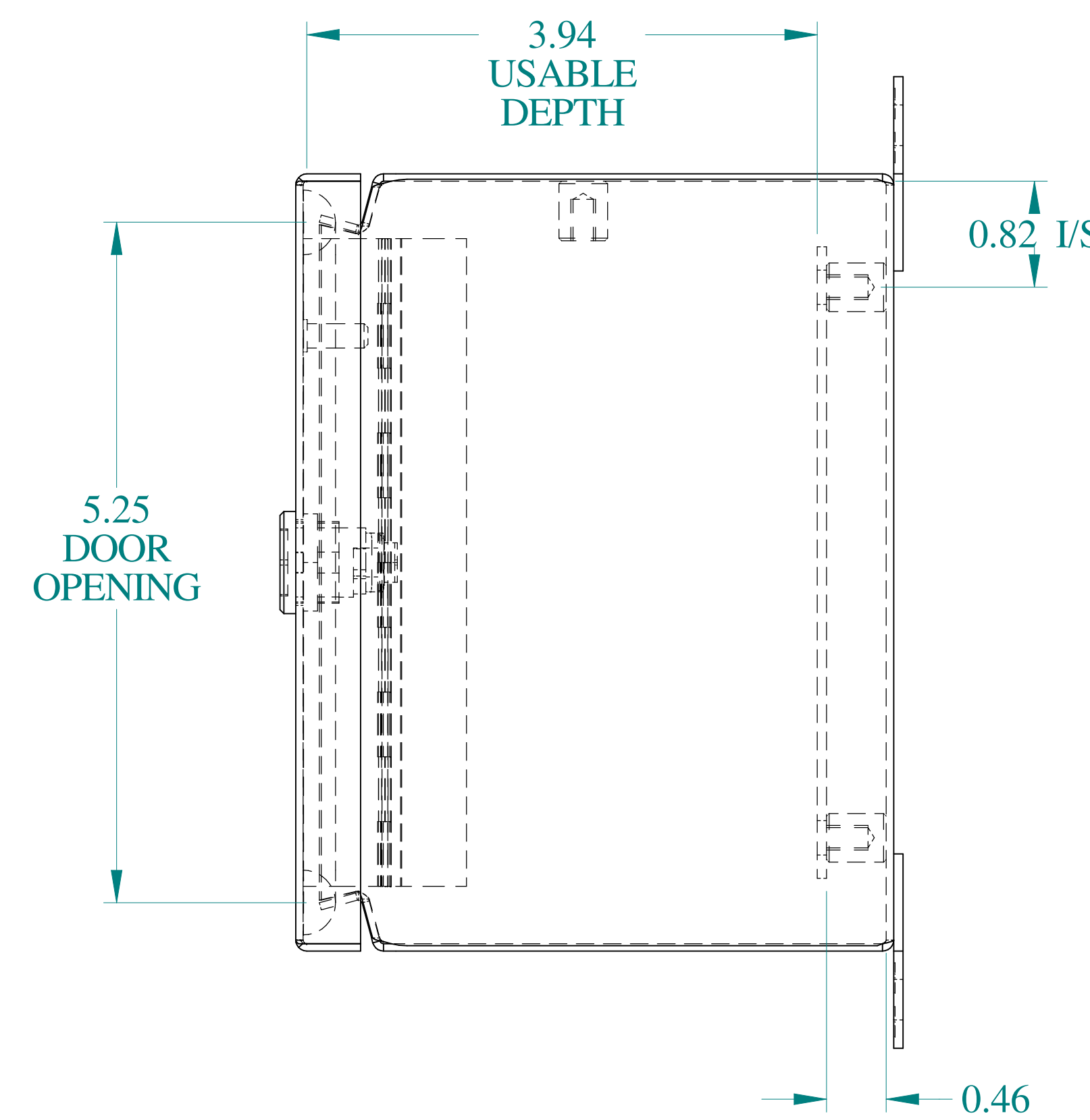
SIDE VIEW
