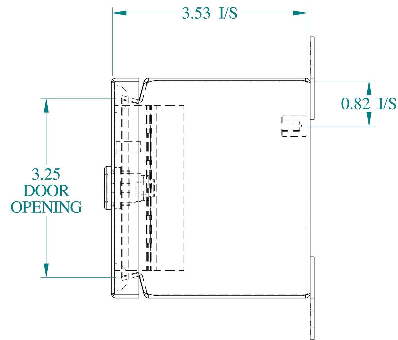
SIDE VIEW
