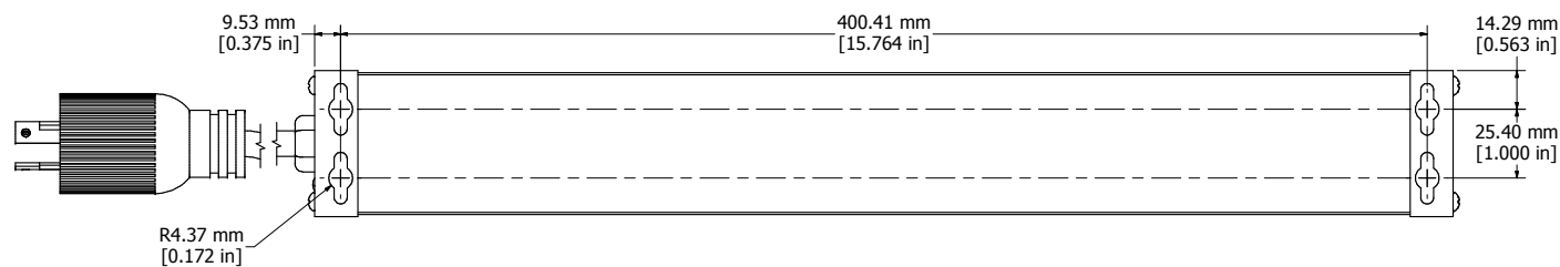
ASSEMBLY - VIEW FROM BOTTOM
