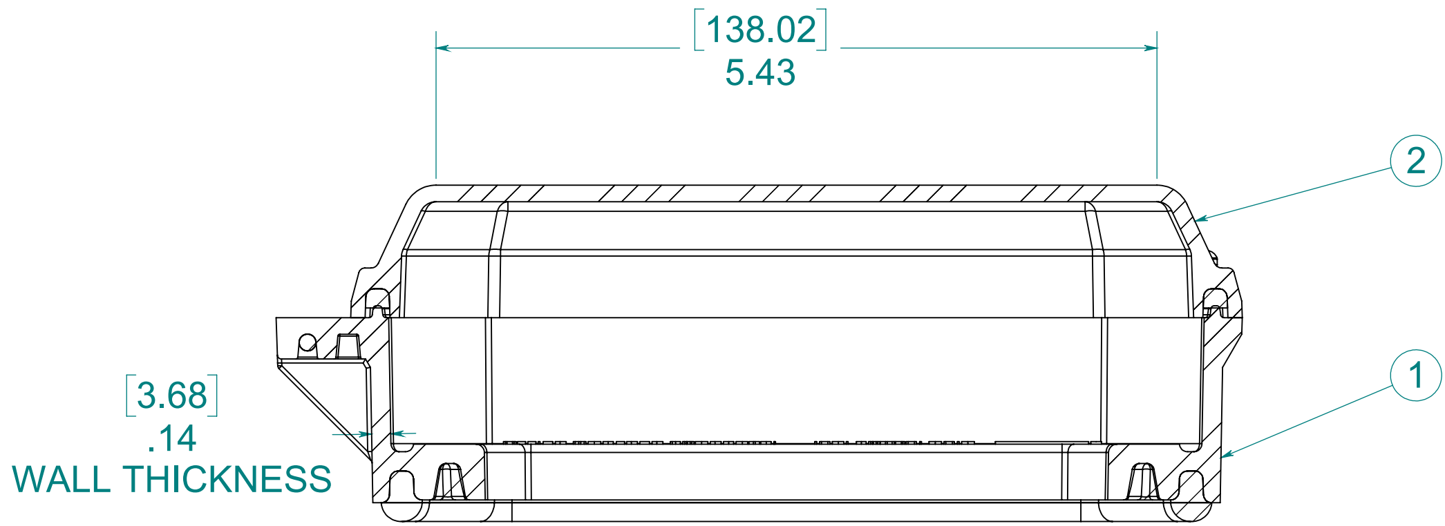
SECTION B-B
