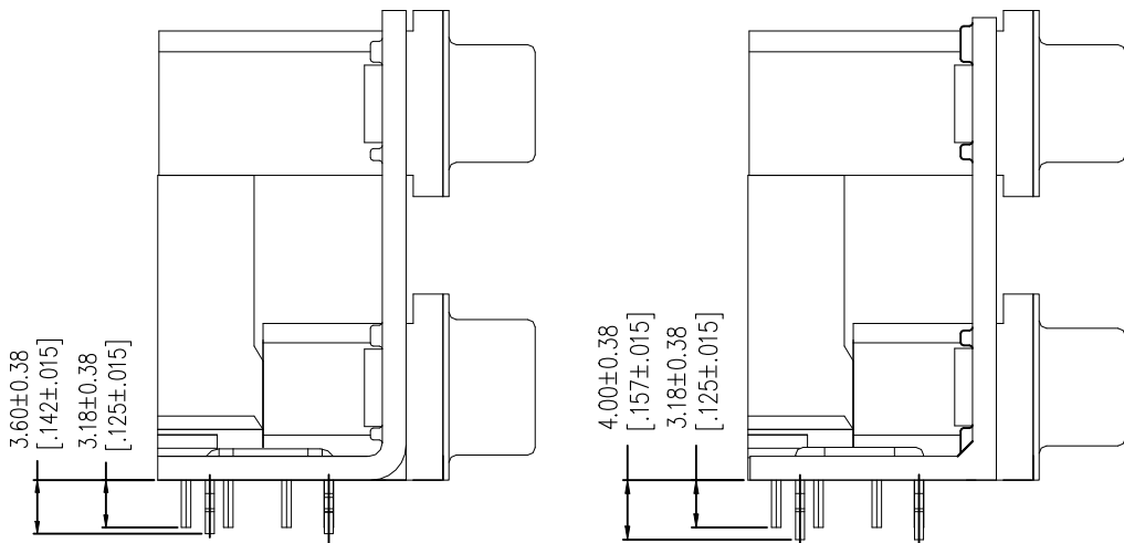
SPCC Alloy Bracket Zinc Alloy Bracket
