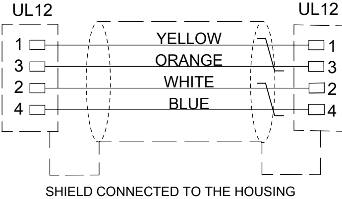
WIRING DIAGRAM (CABLE 12)
