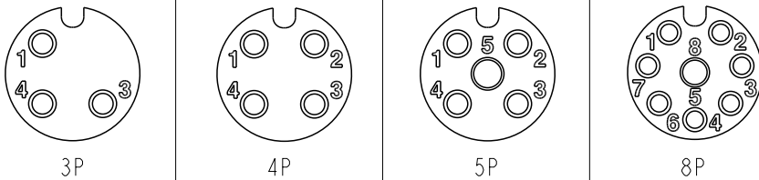
Pin Assignments Front View
