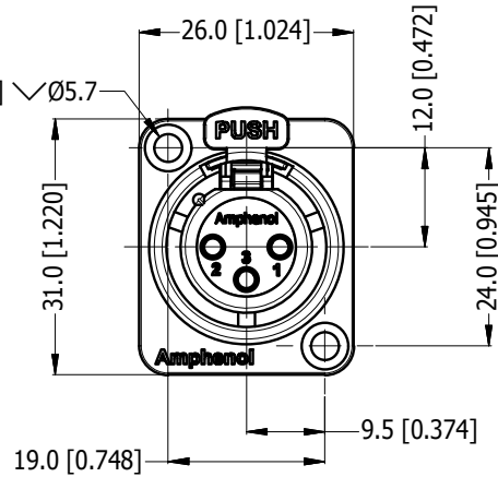
THROUGH HOLE
