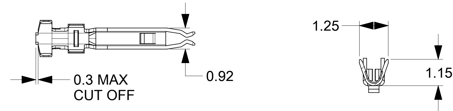
SECTION H-H
