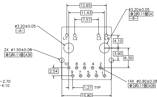
SUGGESTED CUSTOMER BOARD LAYOUT
