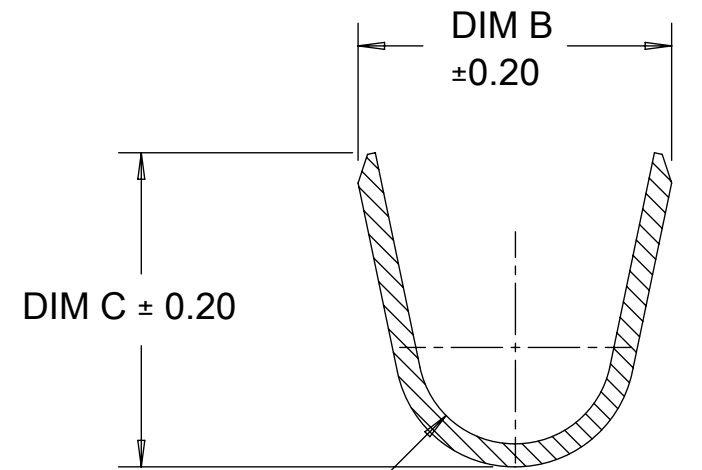
SECTION X-X SCALE 15:1
