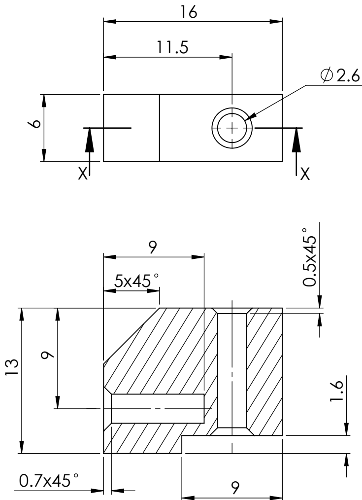
SECTION X-X
