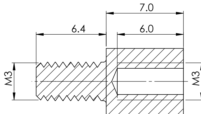
SECTION Y-Y
