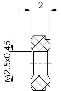
SECTION Y-Y
