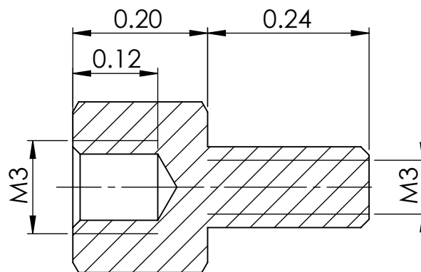
SECTION Y-Y
