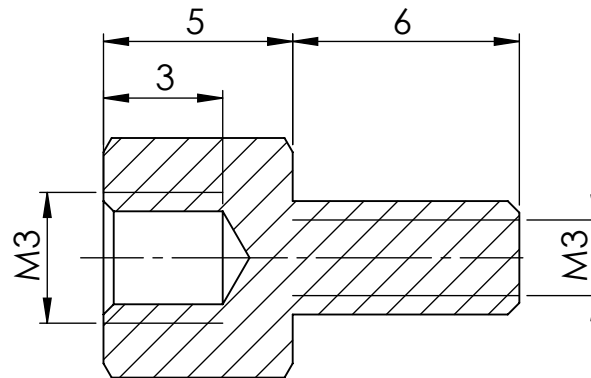
SECTION Y-Y
