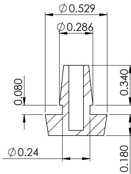
SECTION X-X
