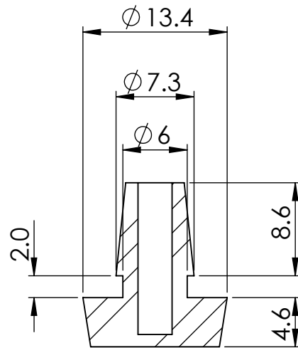
SECTION X-X
