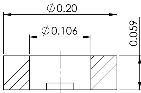
SECTION X-X
