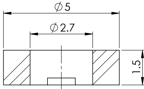
SECTION X-X
