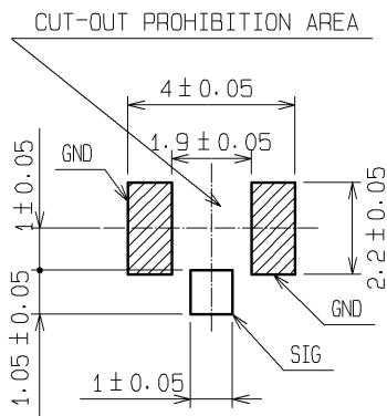
RECOMMENDED PCB LAYOUT (MOUNTING SURFACE SIDE)(5:1)
