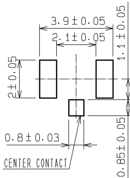
RECOMMENDED METAL MASK DIMENSIONS (5:1) METAL MASK THICKNESS:0.1mm/0.12mm
