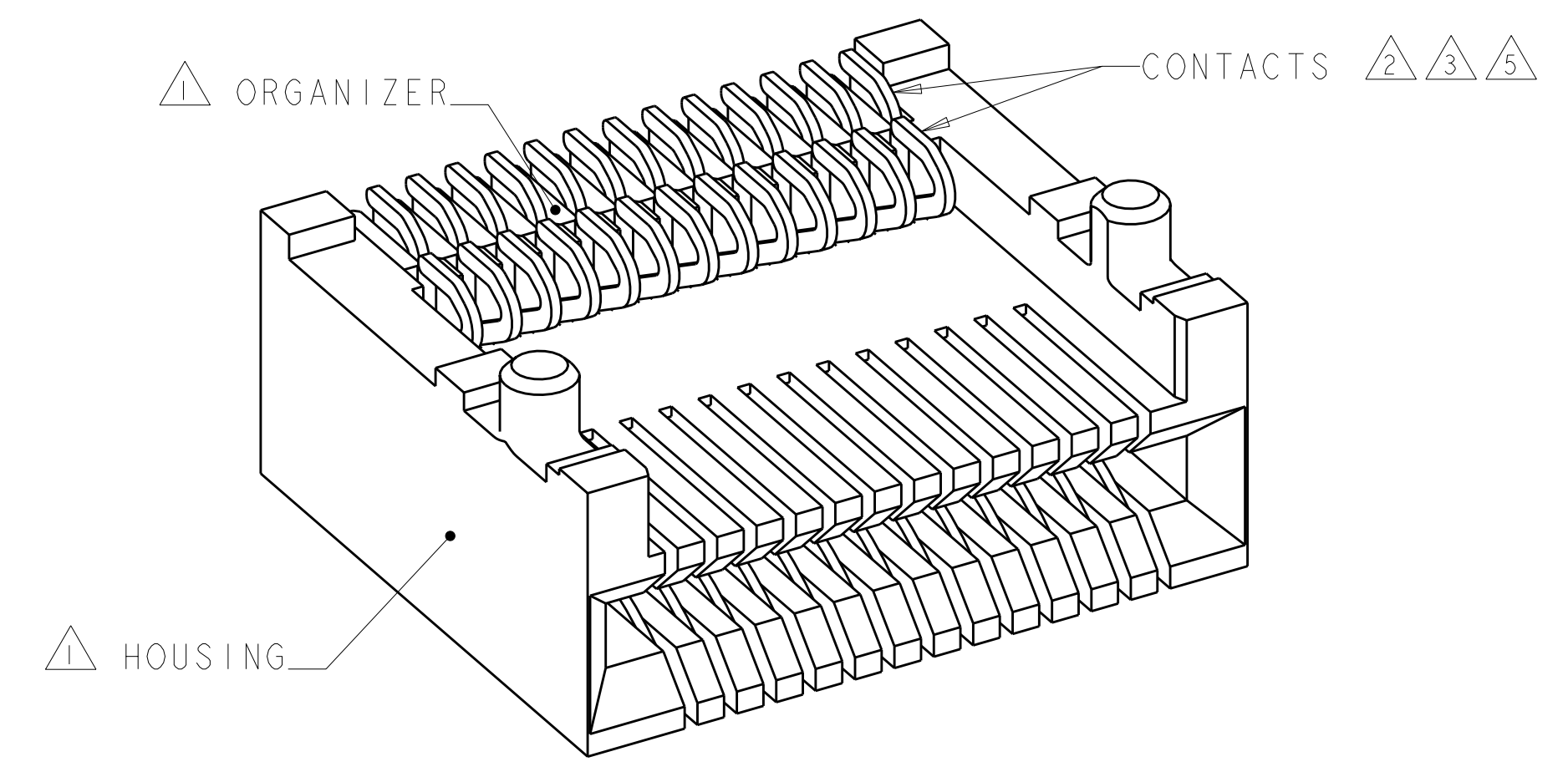
26 POSITION RECEPTACLE SCALE 9:1
