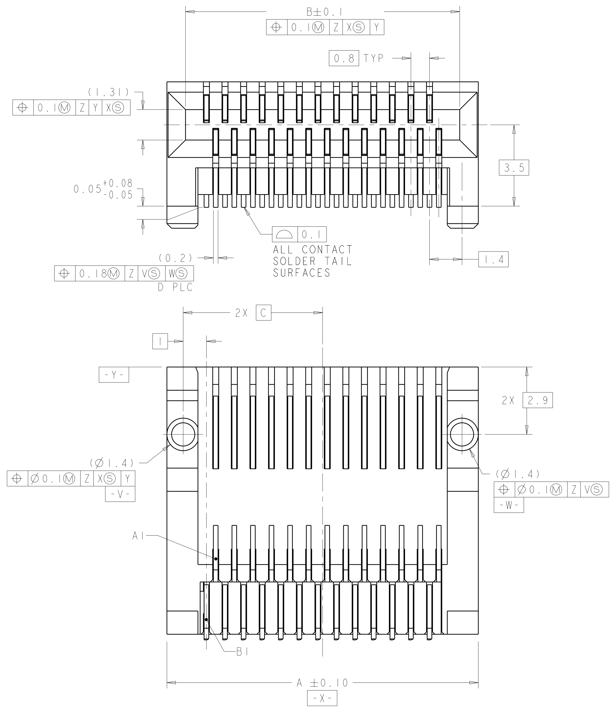
26 POSITION RECEPTACLE SCALE 9:1
