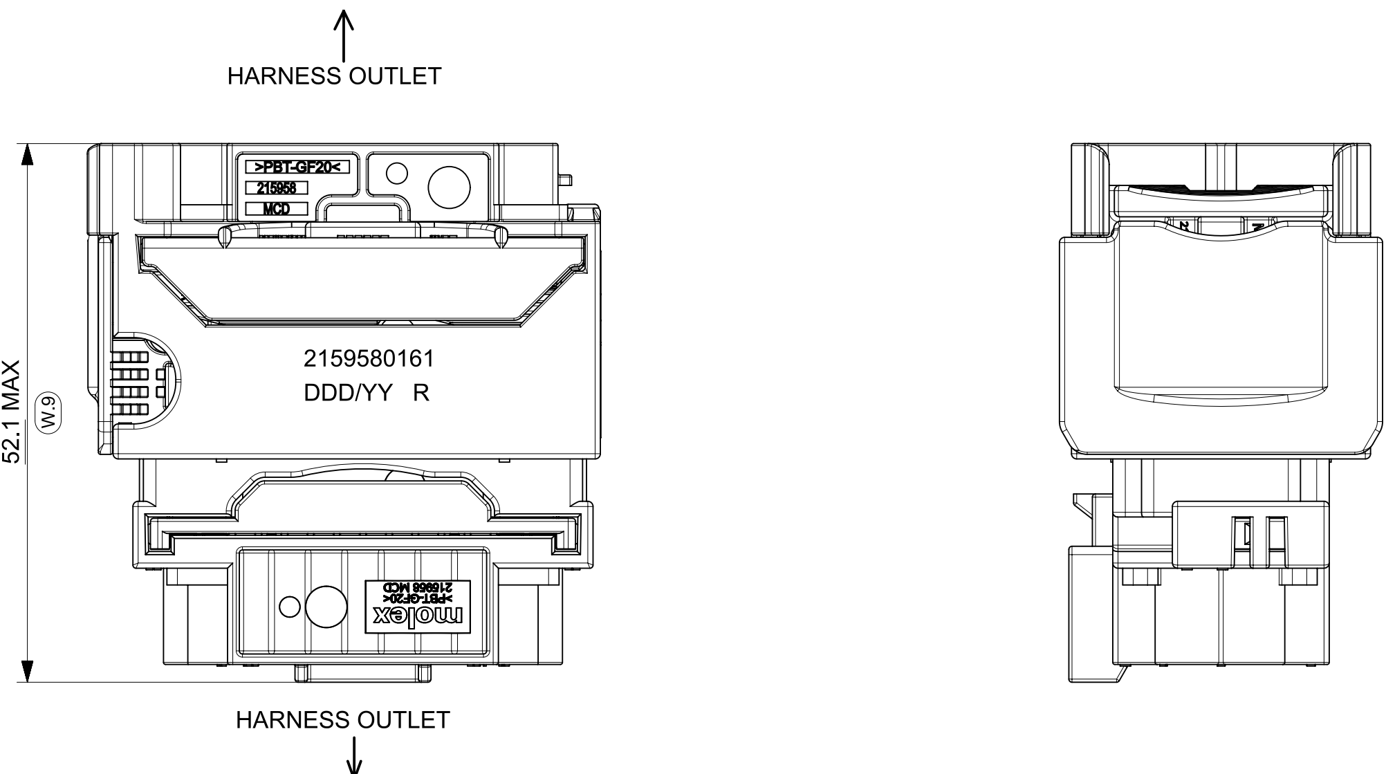
FULLY MATED POSITION
