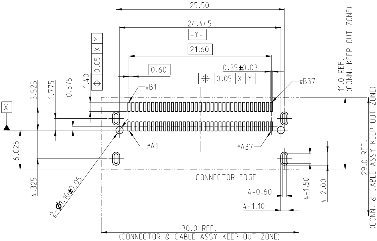
RECOMMENDED PCB LAYOUT- TOP VIEW (GENERAL TOLERANCES: \pm 0.05 )
