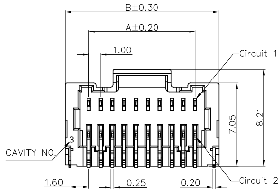
2*10~2*25 Pin, With Four Slot
