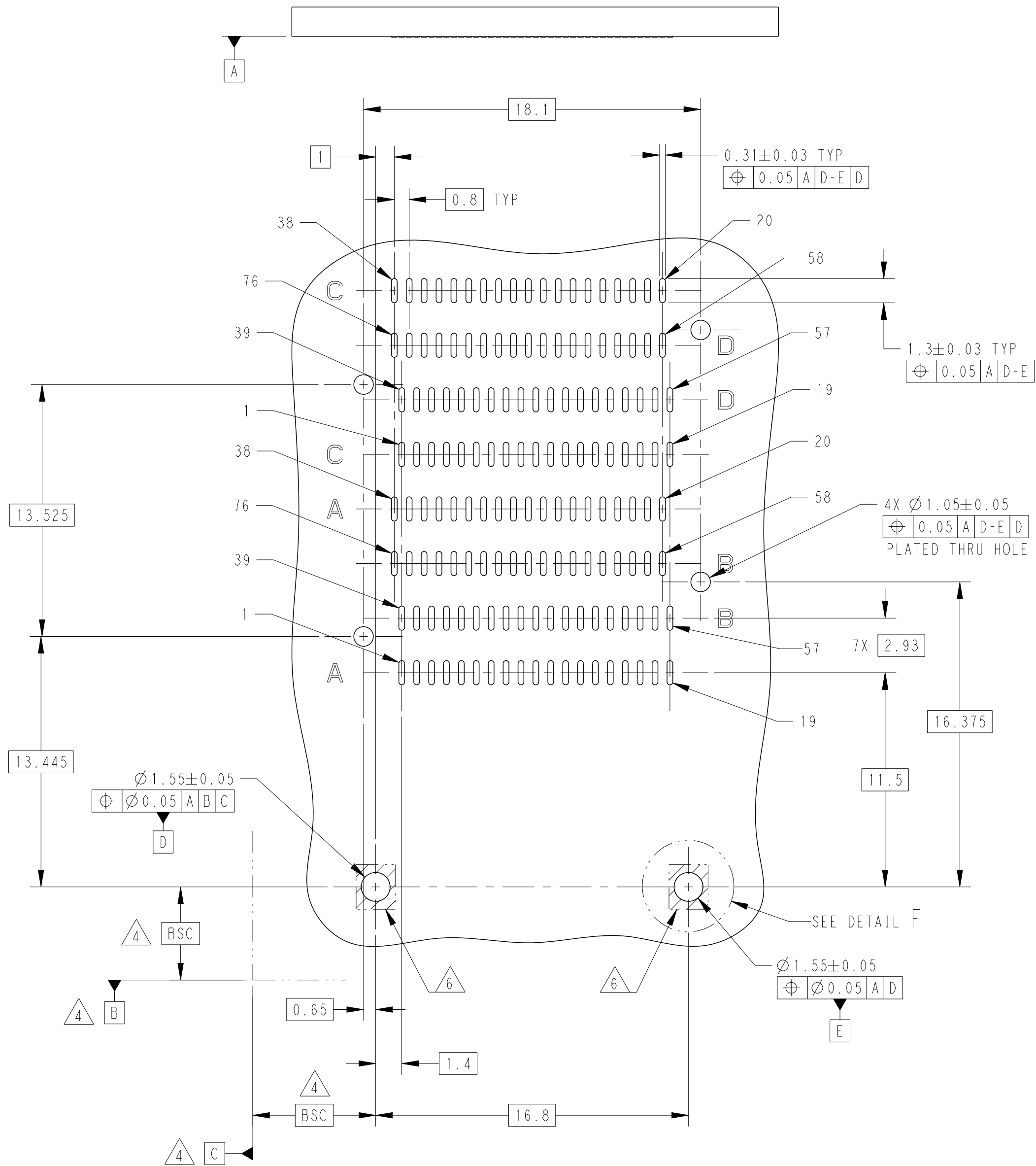
RECOMMENDED PCB LAYOUT SCALE 5:1
