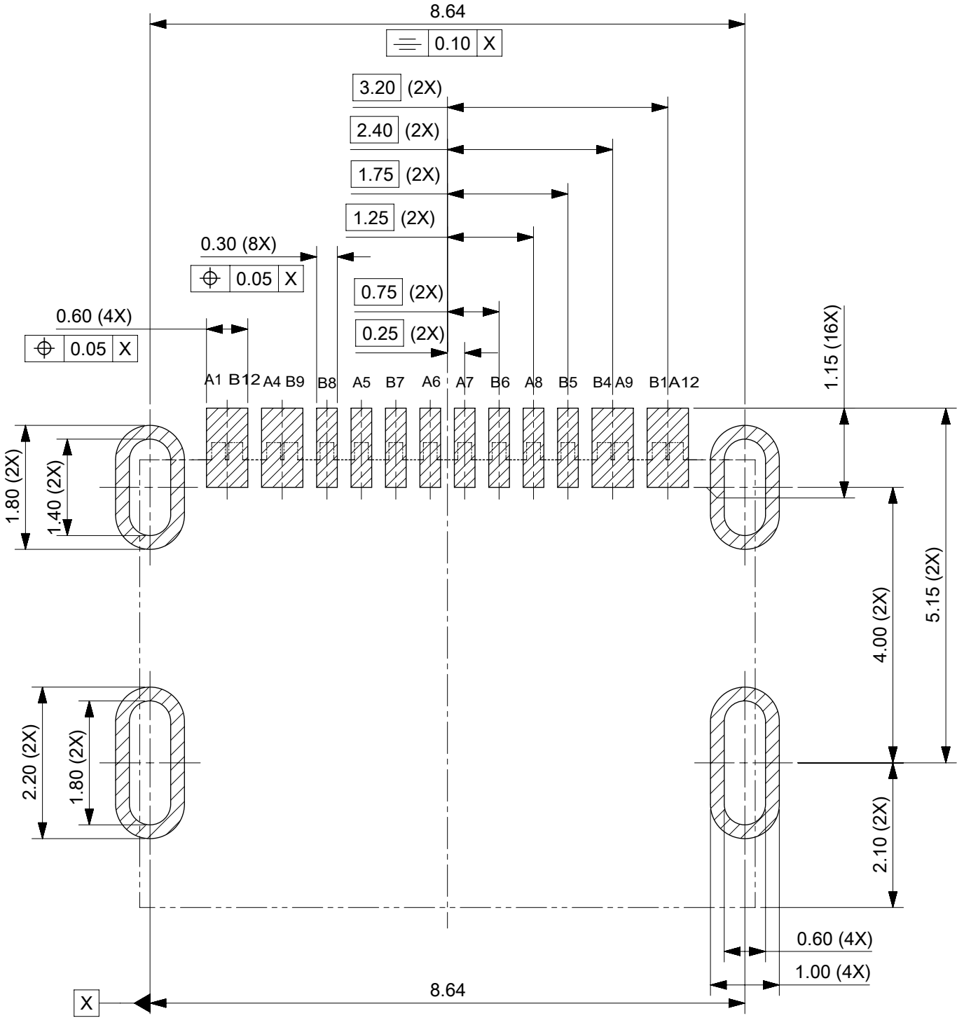
RECOMMENDED PCB LAYOUT(TOP VIEW) THICKNESS 1.20MM;DEFAULT TOLERANCE:±0.05
