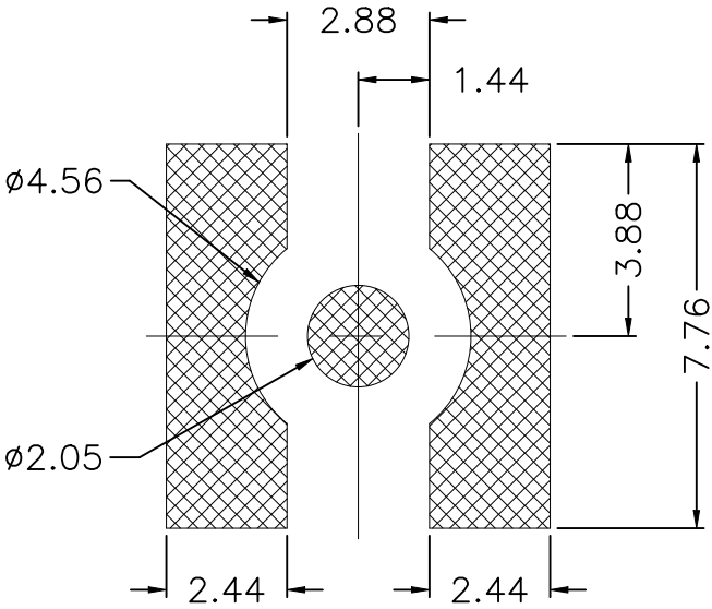
PCB LAYOUT
