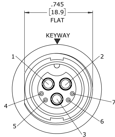
FACE VIEW
