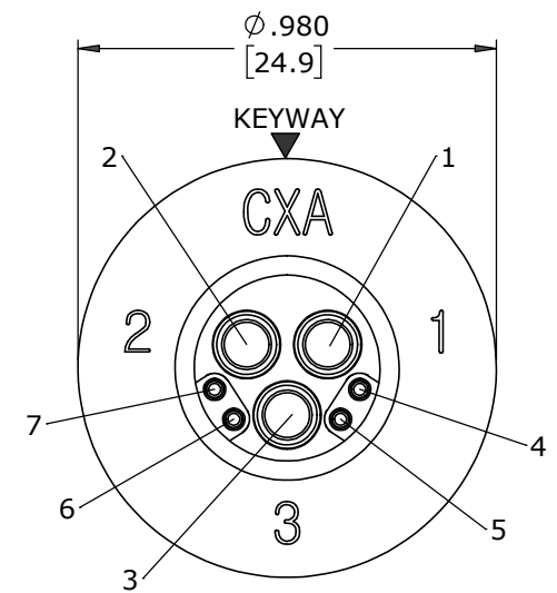
WIRE VIEW
