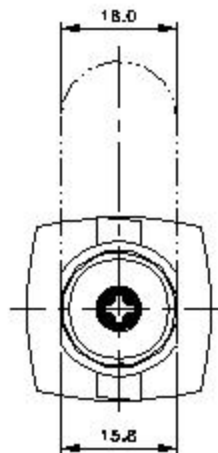
Screwed end
