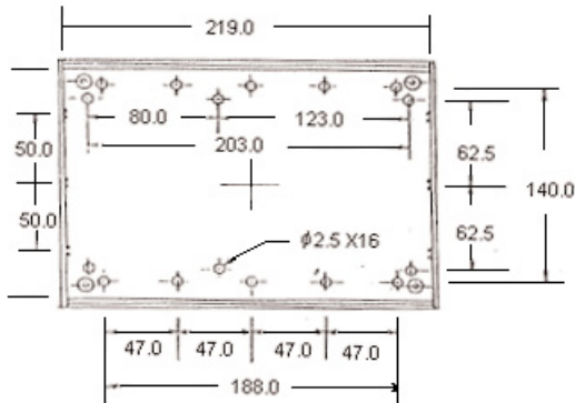
Case Outlines
