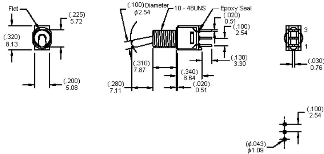
P.C. Mounting Dimensions : Millimetres (Inches)
