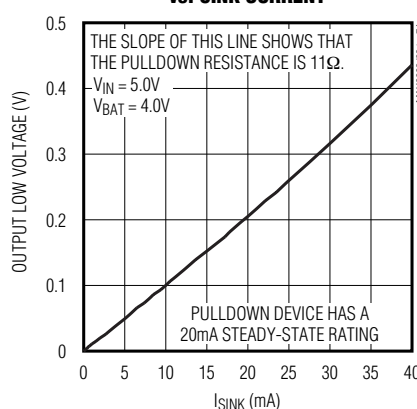
OPEN-DRAIN OUTPUT VOLTAGE LOW vs. SINK CURRENT
