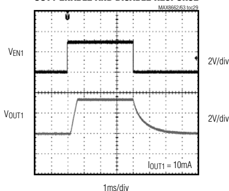
OUT1 ENABLE AND DISABLE RESPONSE
