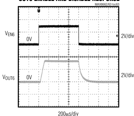
OUT6 ENABLE AND DISABLE RESPONSE
