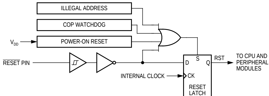
Figure 4-1. Reset Sources
