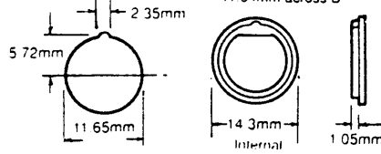
PANEL CUTOUT
