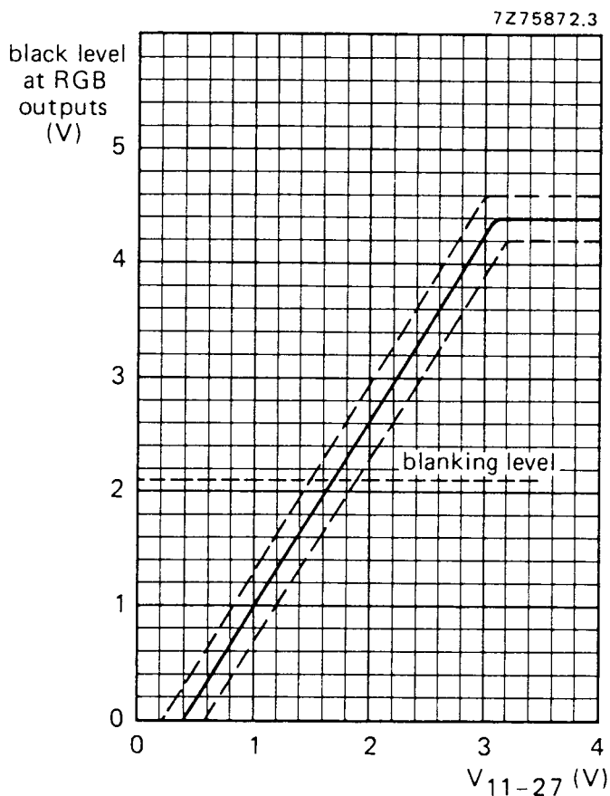
Fig. 5 Brightness control voltage range.
