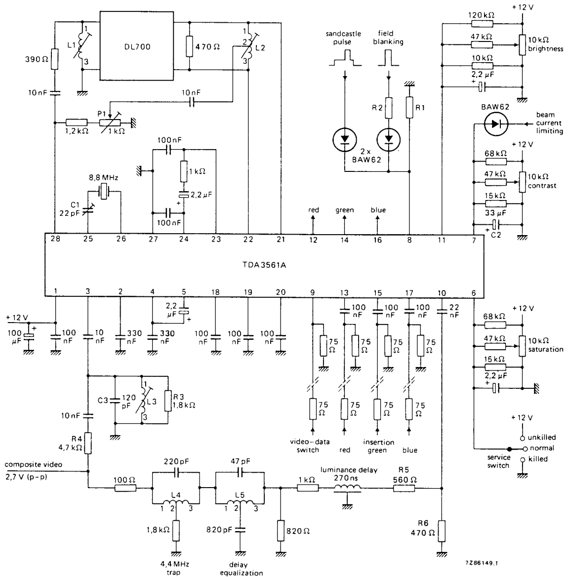
Fig. 6 Application circuit.
