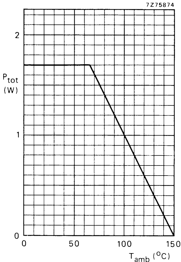
Fig. 2 Power derating curve.
