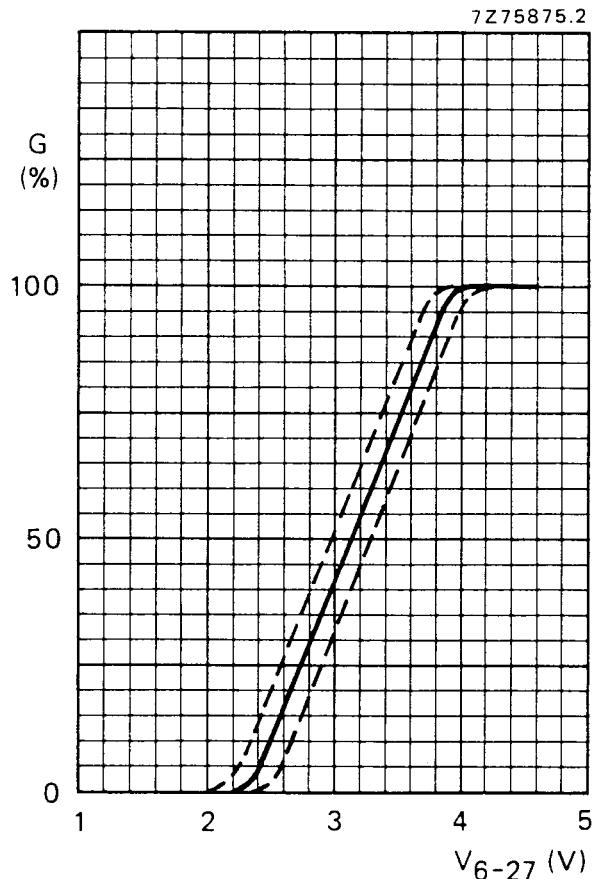
Fig. 4 Saturation control voltage range.
