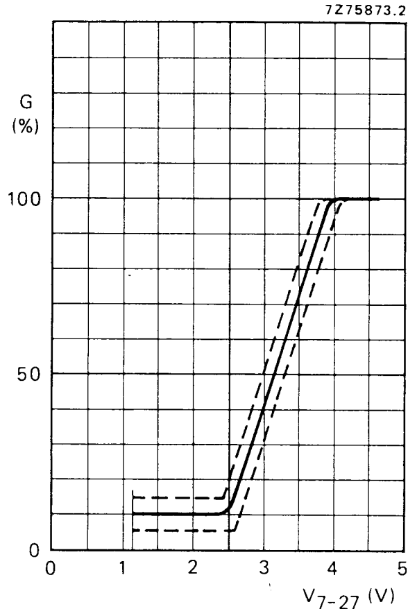
Fig. 3 Contrast control voltage range.
