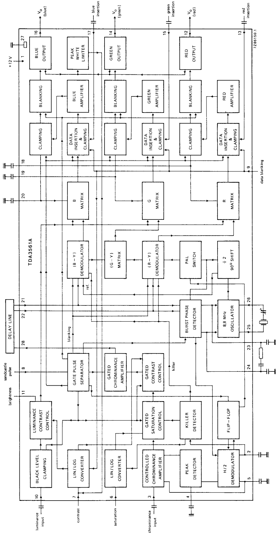
Fig. 1 Block diagram.
