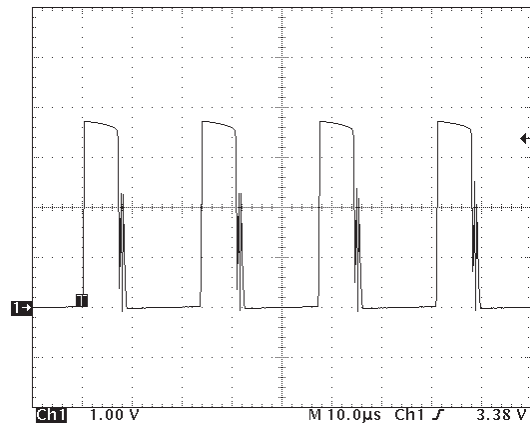
Figure 3. Switching waveform
