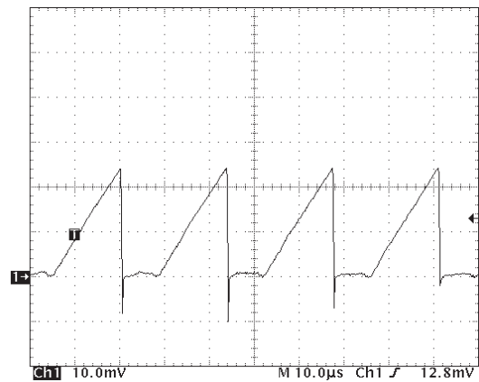
Figure 4. I_SENSE threshold
