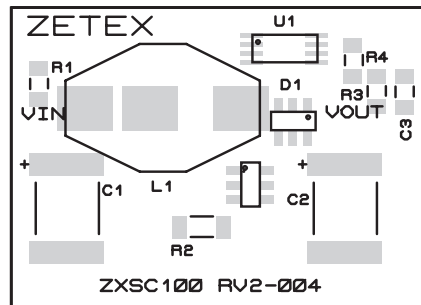
Top silk
