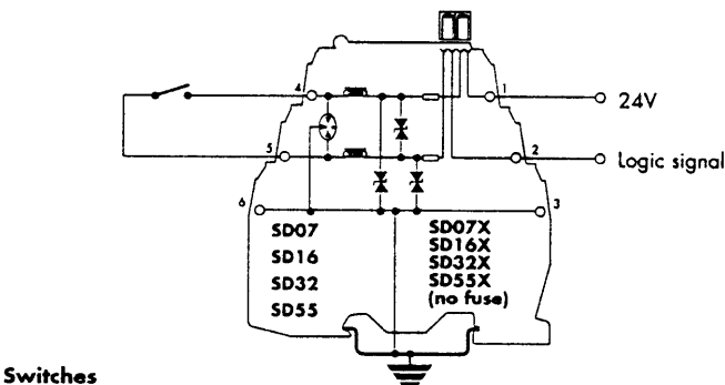
Switches
