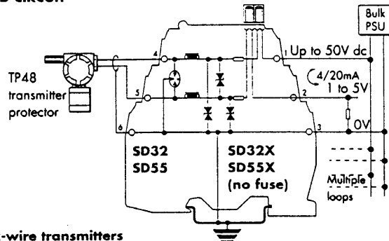
2-wire transmitters
