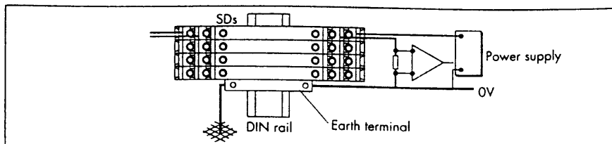
PLC/I/O systems
