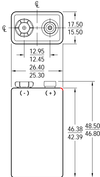
Dimensions (mm)
