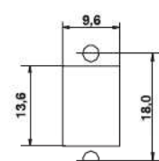
Hole pattern
