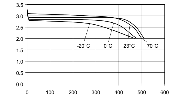
Temperature performance Load 47 kΩ
