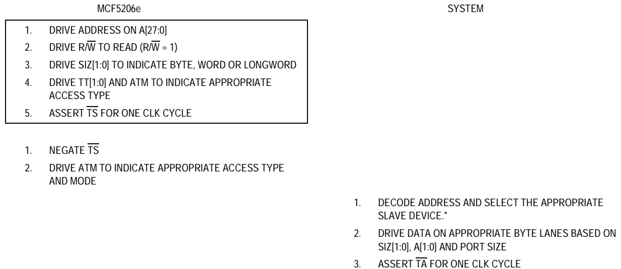
Figure 6-4. Byte-, Word-, and Longword-Read Transfer Flowchart
