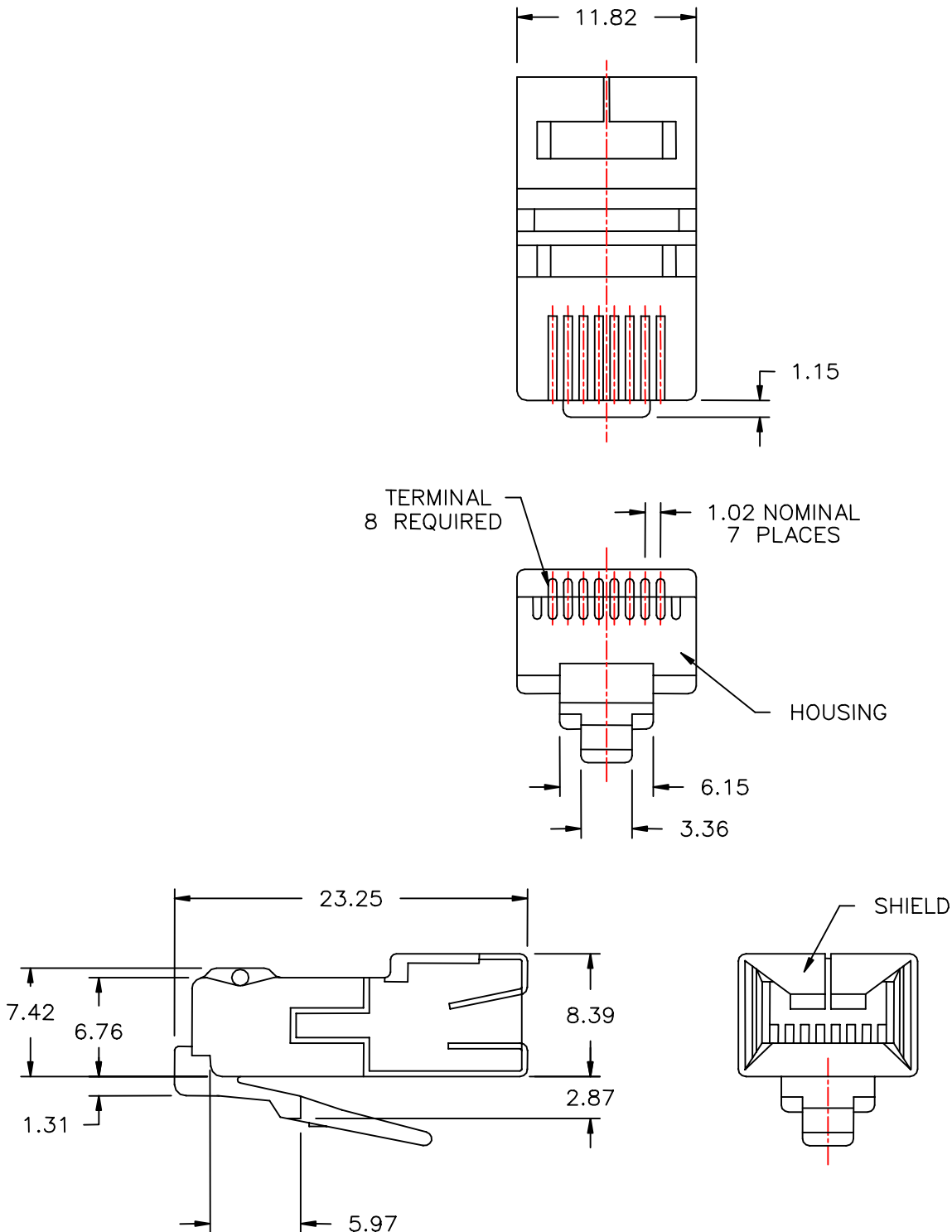
Figure 2 – Unshielded Mating Plug
