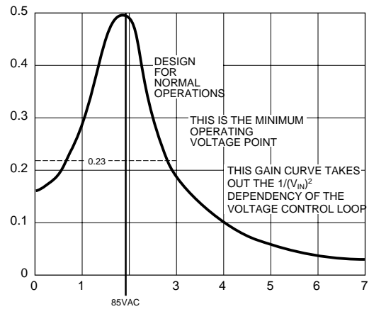
Figure 6. K-factor. Gain Modulator gain with respect to the voltage at VRMS.
