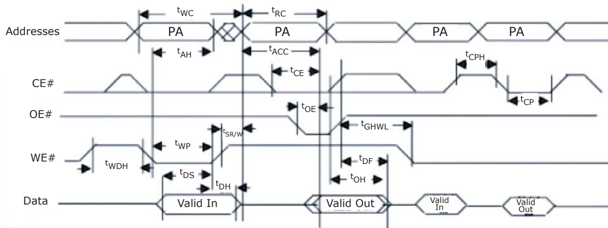
Figure 15.7 Back to Back Read/Write Cycle Timing
