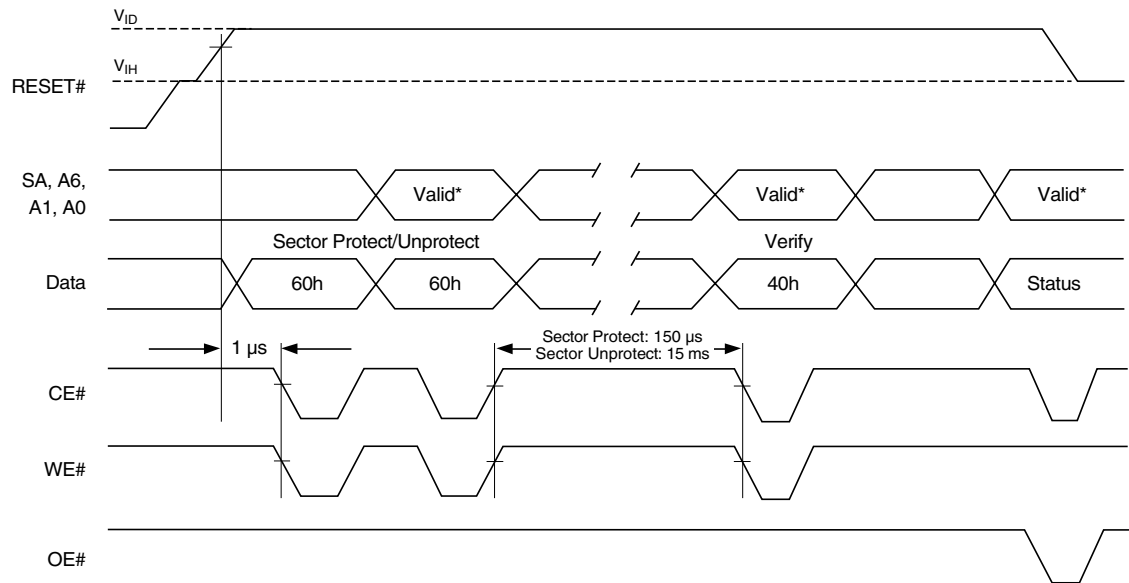
Figure 15.12 Sector Protect/Unprotect Timing Diagram
