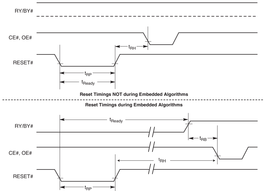
Figure 15.2 RESET# Timings
