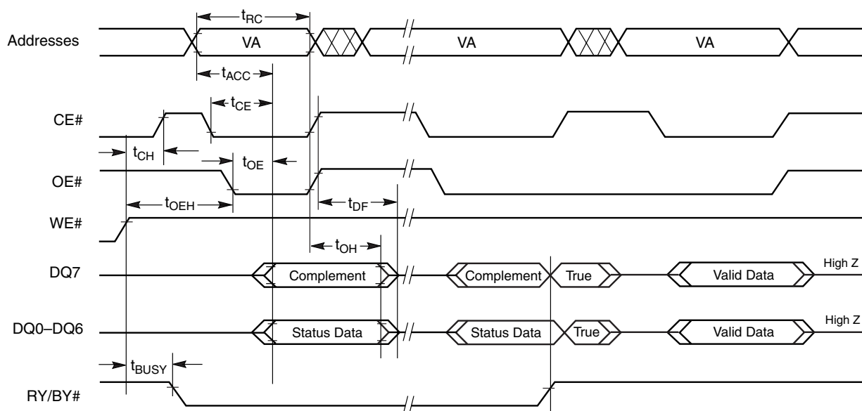
Figure 15.8 Data# Polling Timings (During Embedded Algorithms)
