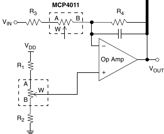
FIGURE 8-3: Trimming Offset and Gain in an Inverting Amplifier.
