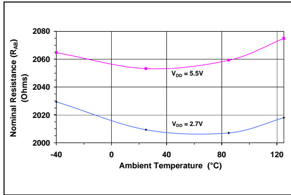
FIGURE 2-11: 2.1 k \Omega – Nominal Resistance ( \Omega ) vs. Ambient Temperature and V_{DD} .
