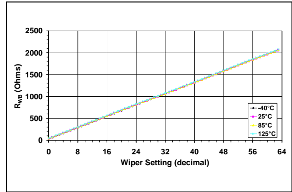
FIGURE 2-12: 2.1 k \Omega – R_{WB} ( \Omega ) vs. Wiper Setting and Ambient Temperature.
