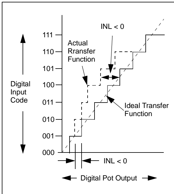
FIGURE 6-5: INL Accuracy.
