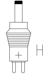
Hohlstecker/ hollowplug ø2,1xø5x12mm
