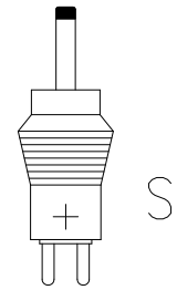
Hohlstecker/ hollowplug ø1,7xø4x10mm
