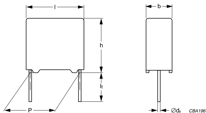
Fig.3 Outline.
