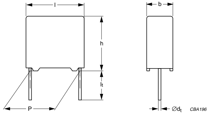
Fig.1 Simplified outlines.
