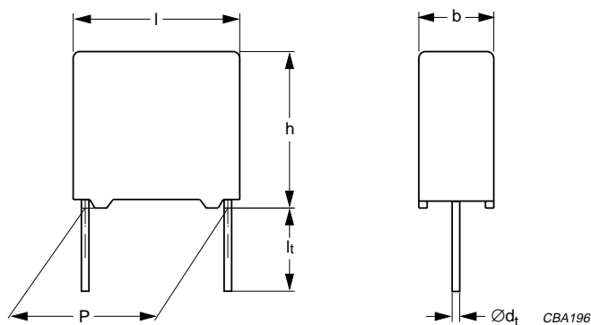
Fig.4 Outline.
