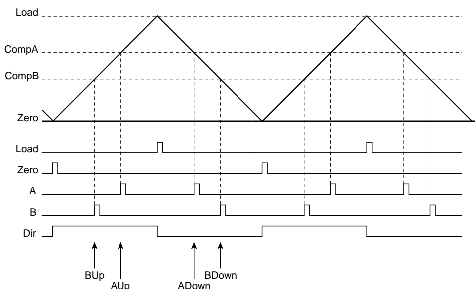
Figure 18-3. PWM Count-Up/Down Mode
