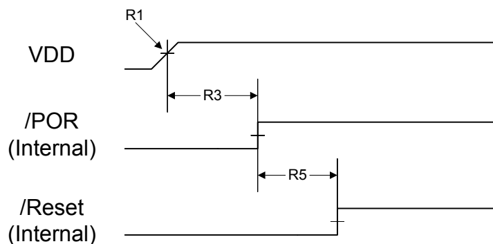
Figure 23-13. Brown-Out Reset Timing
