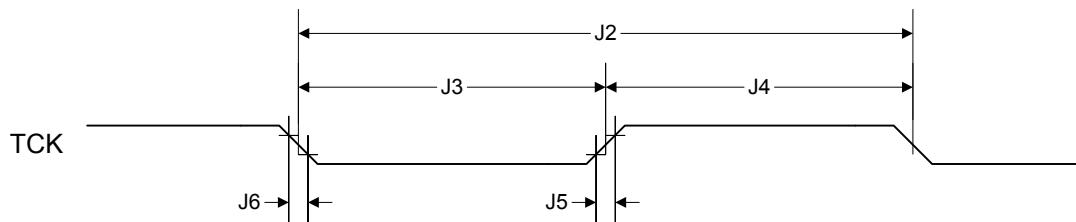
Figure 23-8. JTAG Test Clock Input Timing
