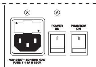
Fig. 2.17: Voltage supply and fuse
