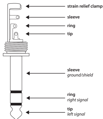
Fig. 4.6: ¼" TRS connector for headphones
