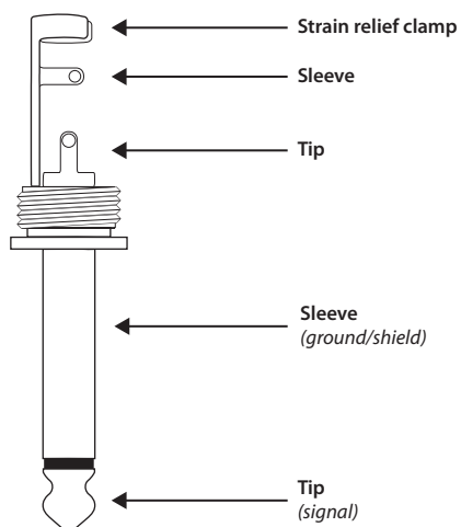
Fig. 4.3: ¼" TS connector
