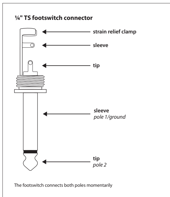
Fig. 4.1: 1/4" TS footswitch connector
