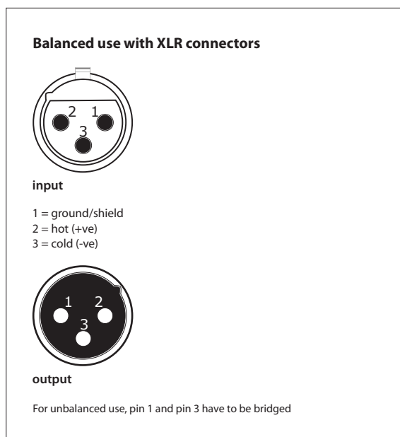
Fig. 4.2: XLR connections
