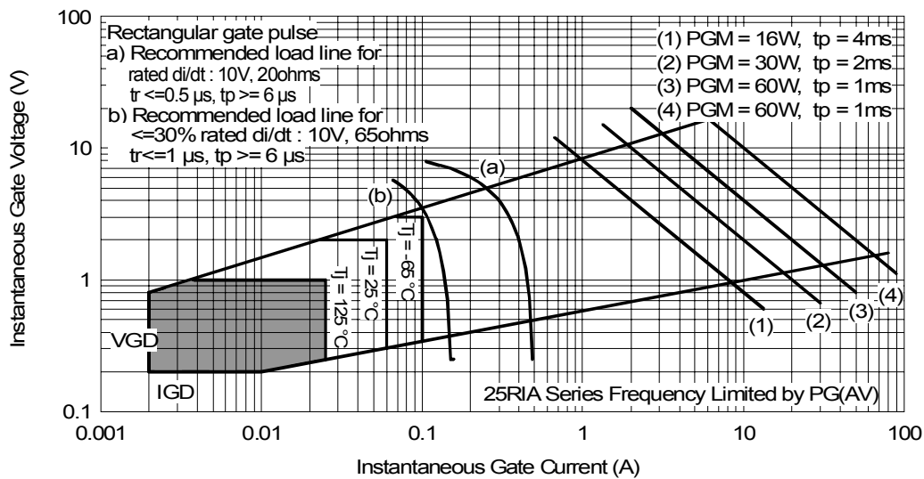
Fig. 16 - Gate Characteristics
