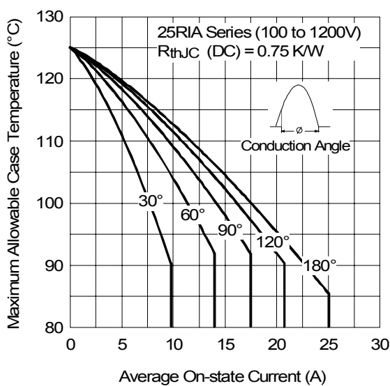
Fig. 1 - Current Ratings Characteristic
