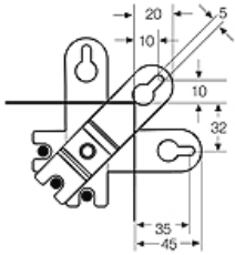
Dimension drawing
